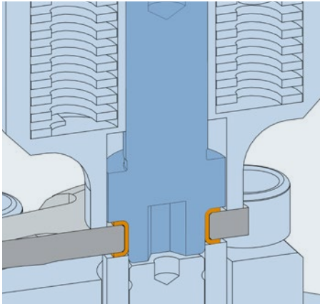
Bushings
